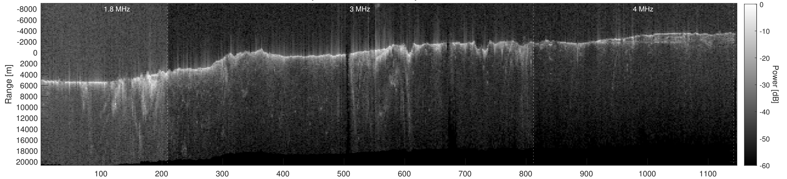
Orbit 4874, Depth-Corrected Cluttergram
