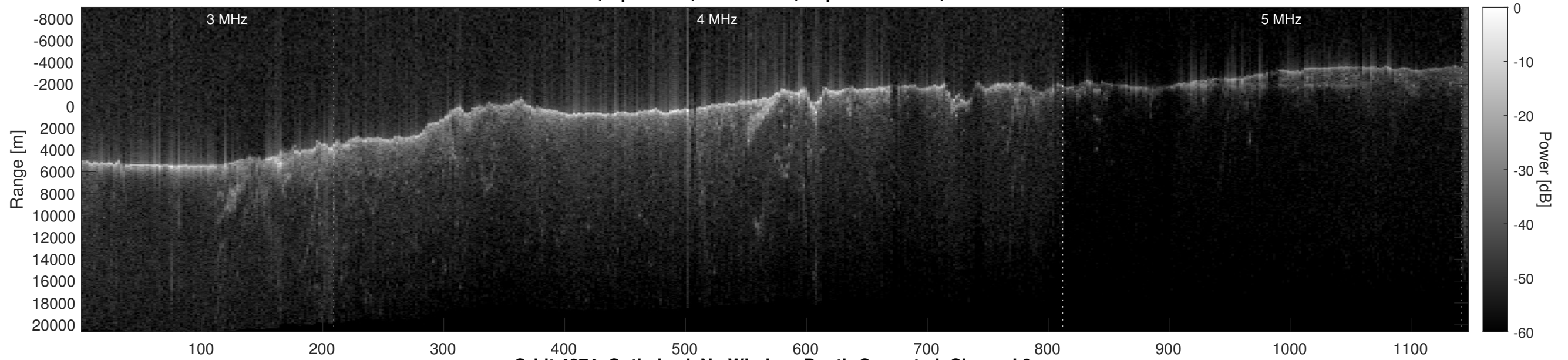
Orbit 4874, Optimized, No Window, Depth-Corrected, Channel 2
