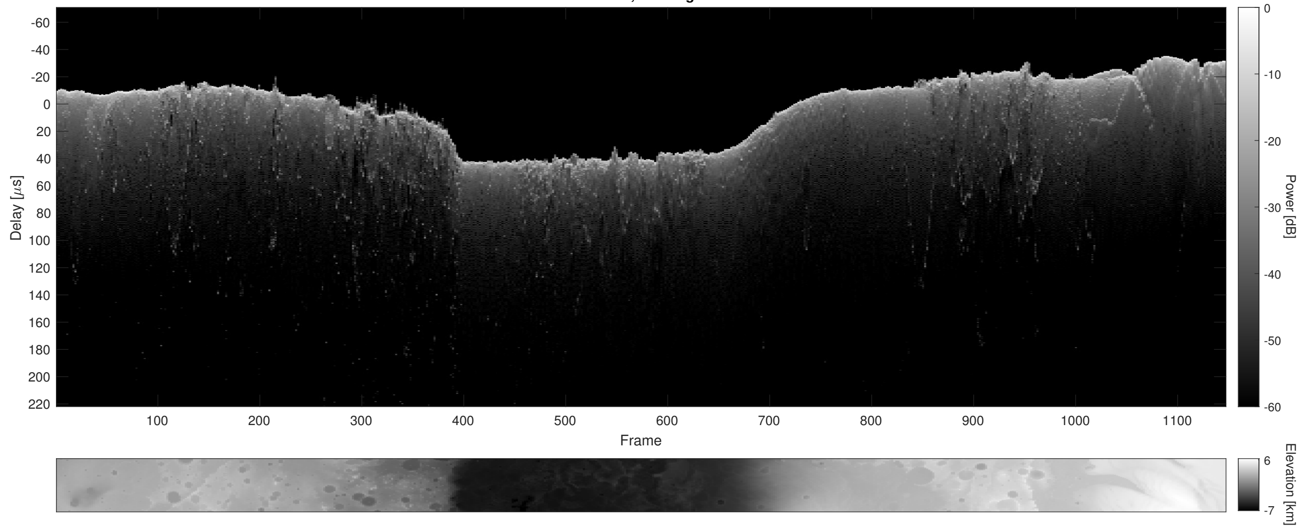
Orbit 4875, Cluttergram
