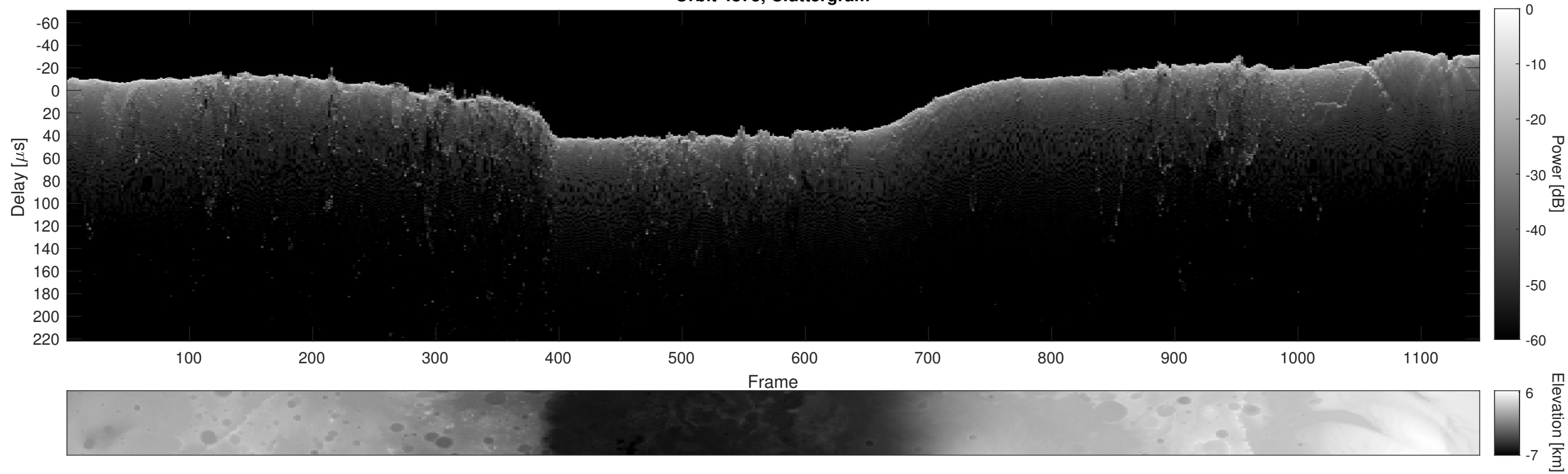
Orbit 4875, Cluttergram
