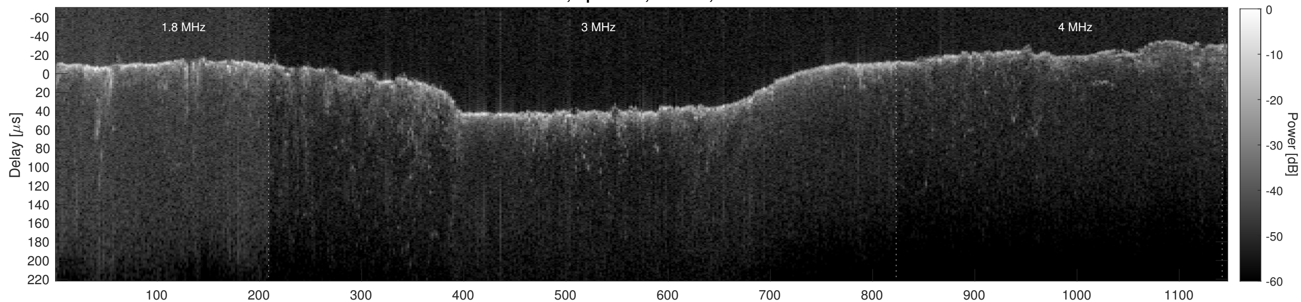
Orbit 4875, Cluttergram
