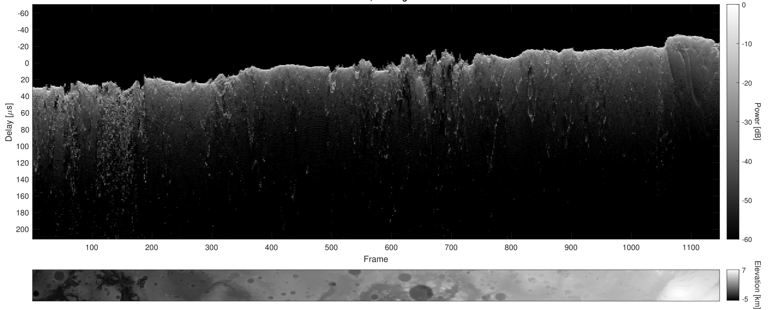
Orbit 4876, Cluttergram
