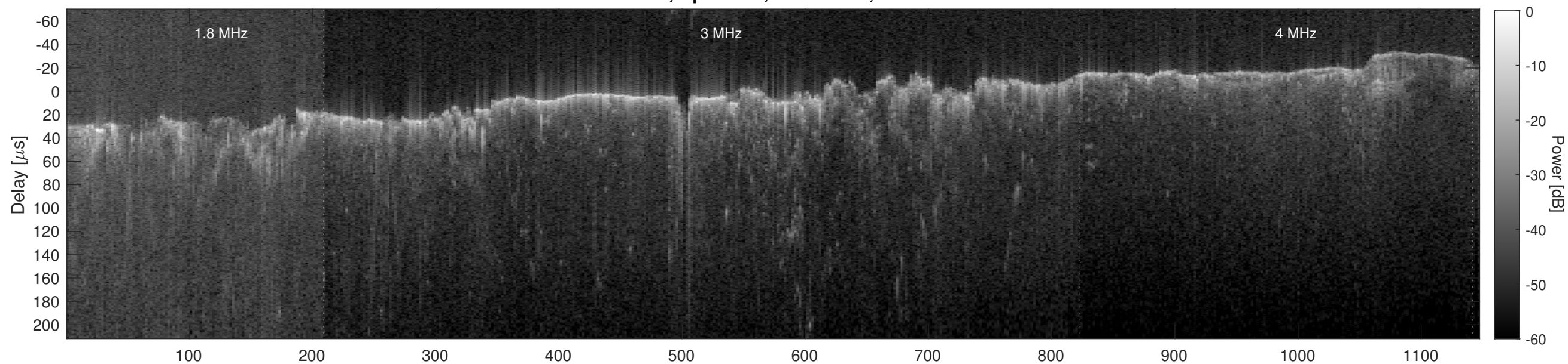
Orbit 4876, Cluttergram
