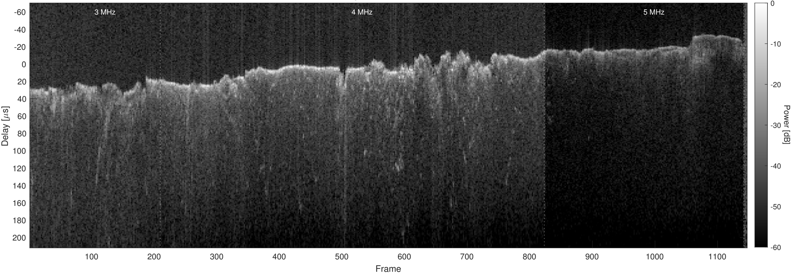
Orbit 4876, Optimized, Window, Channel 2
