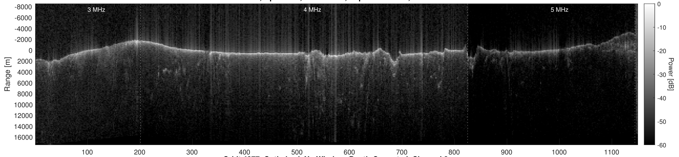
Orbit 4877, Optimized, No Window, Depth-Corrected, Channel 2
