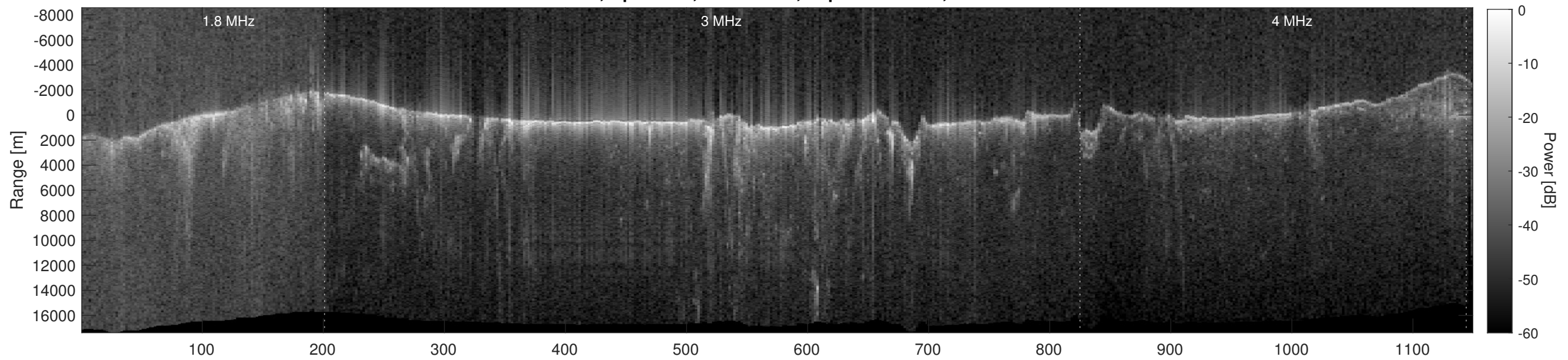
Orbit 4877, Depth-Corrected Cluttergram
