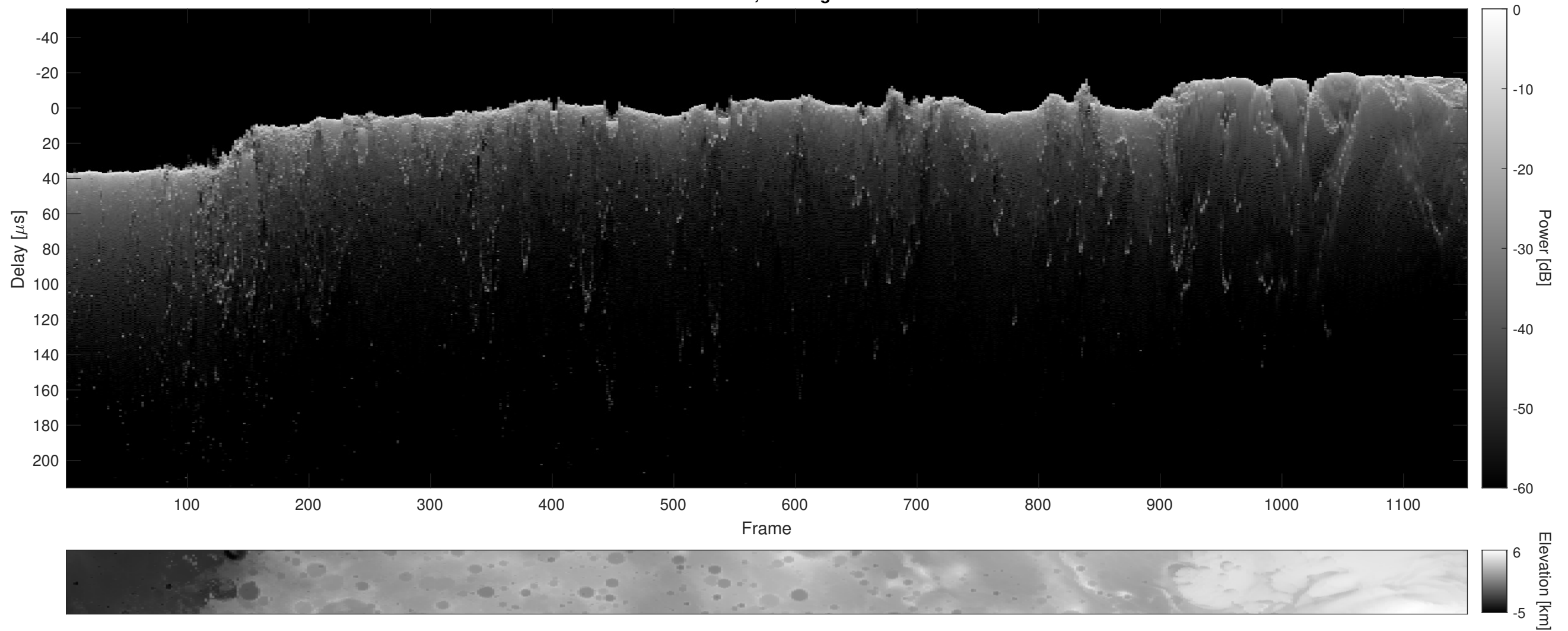
Orbit 4878, Cluttergram
