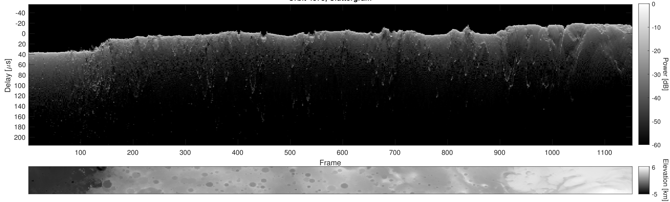
Orbit 4878, Cluttergram
