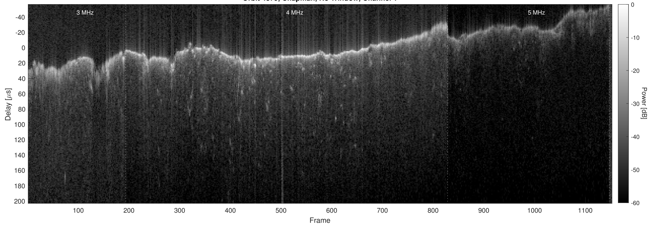
Orbit 4879, Chapman, No Window, Channel 2
