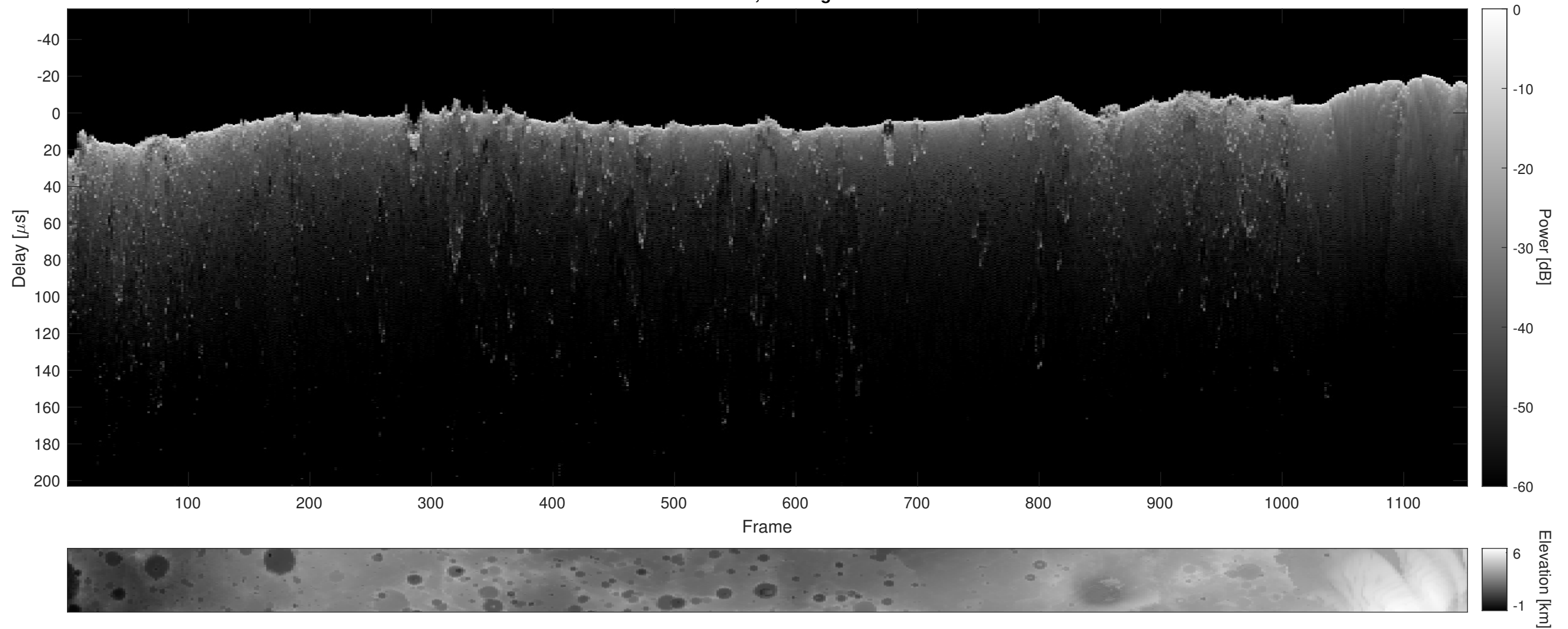
Orbit 4879, Cluttergram
