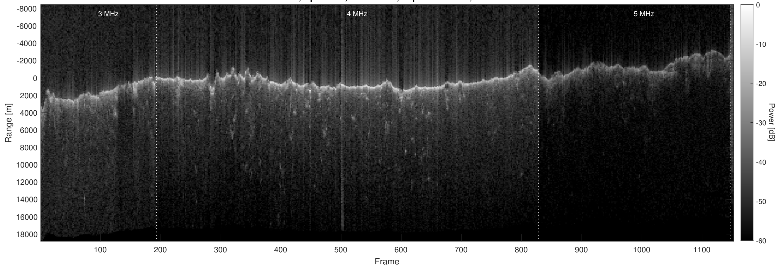
Orbit 4879, Optimized, No Window, Depth-Corrected, Channel 2
