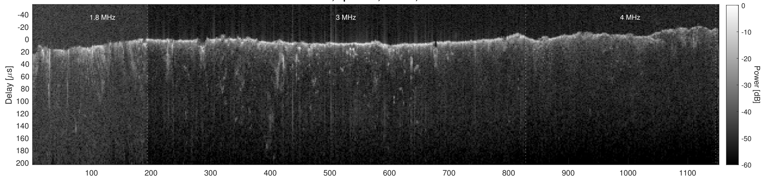
Orbit 4879, Cluttergram
