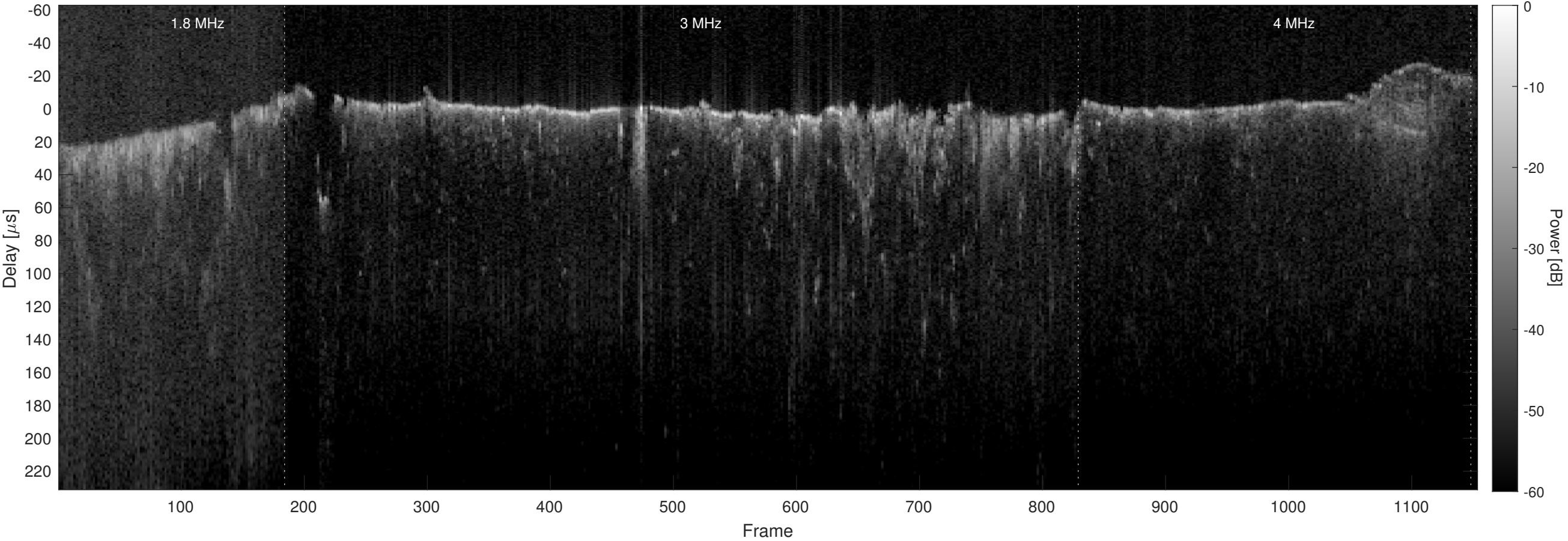
Orbit 4880, Optimized, Window, Channel 2
