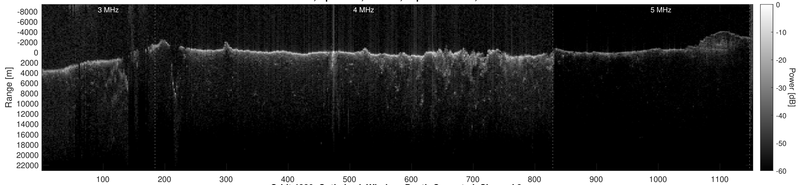
Orbit 4880, Optimized, Window, Depth-Corrected, Channel 2
