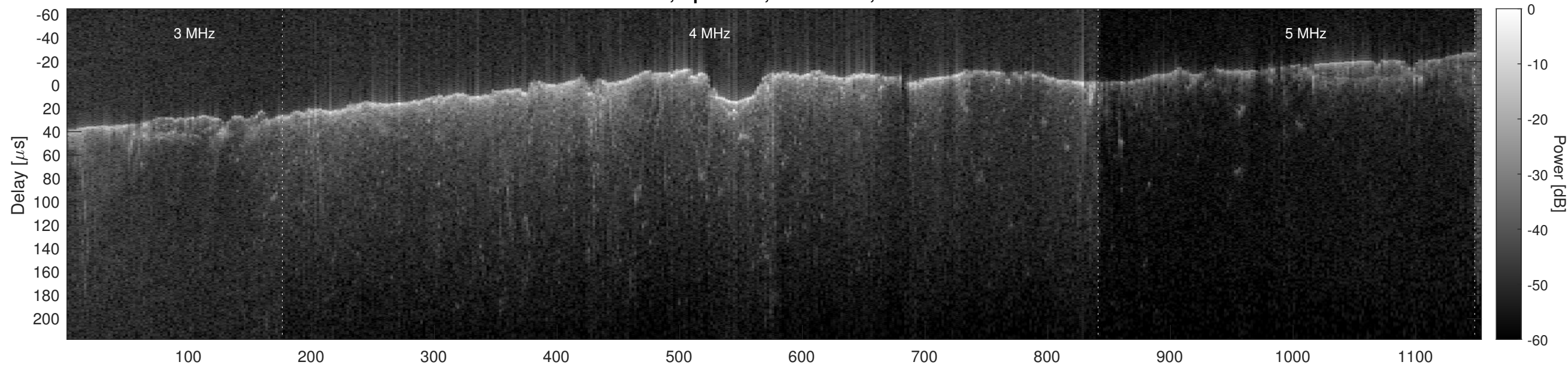
Orbit 4881, Optimized, No Window, Channel 2
