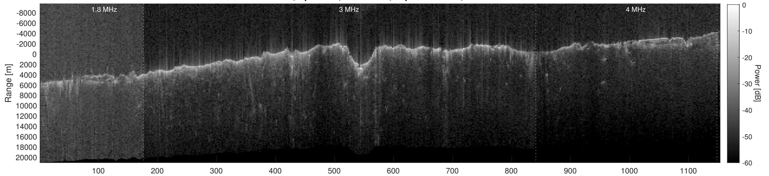
Orbit 4881, Depth-Corrected Cluttergram
