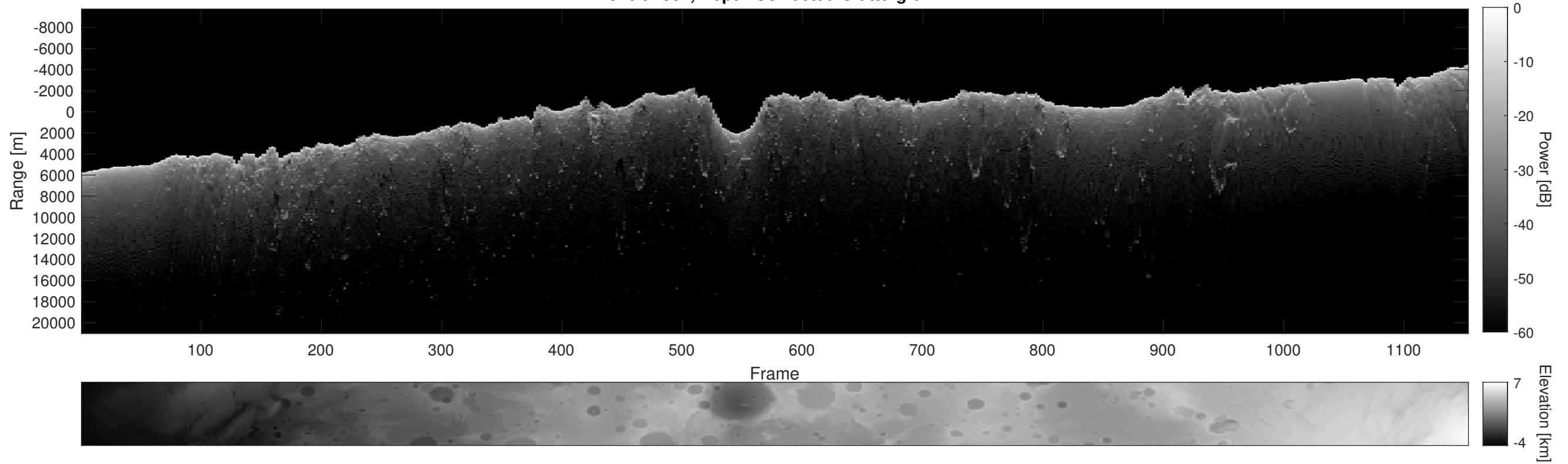
Orbit 4881, Depth-Corrected Cluttergram
