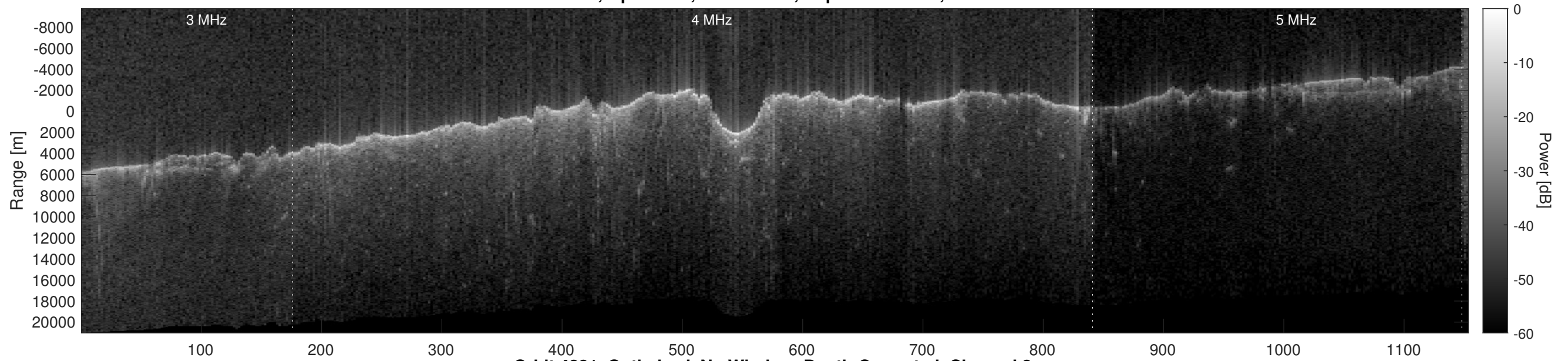
Orbit 4881, Optimized, No Window, Depth-Corrected, Channel 2
