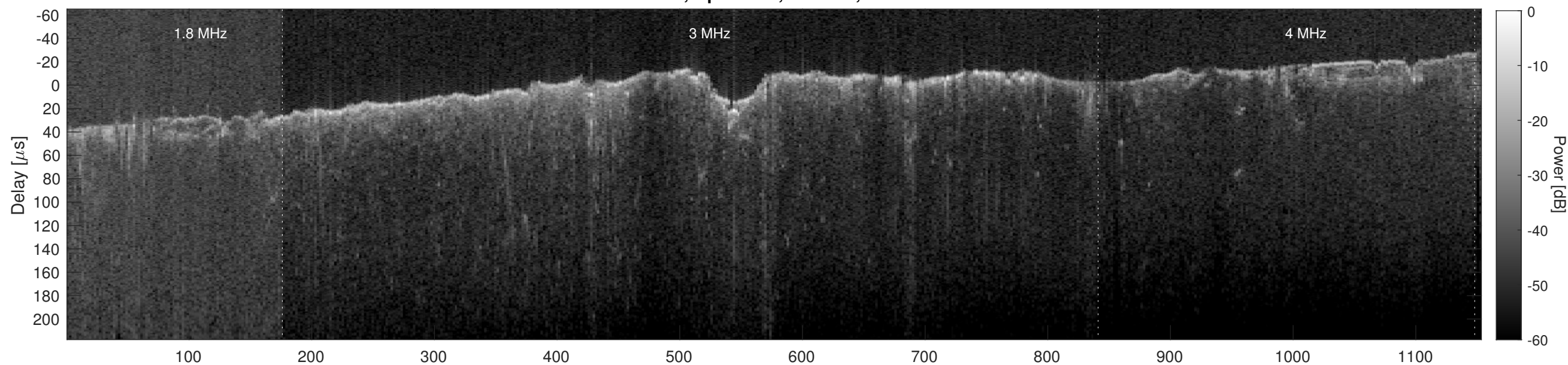
Orbit 4881, Cluttergram
