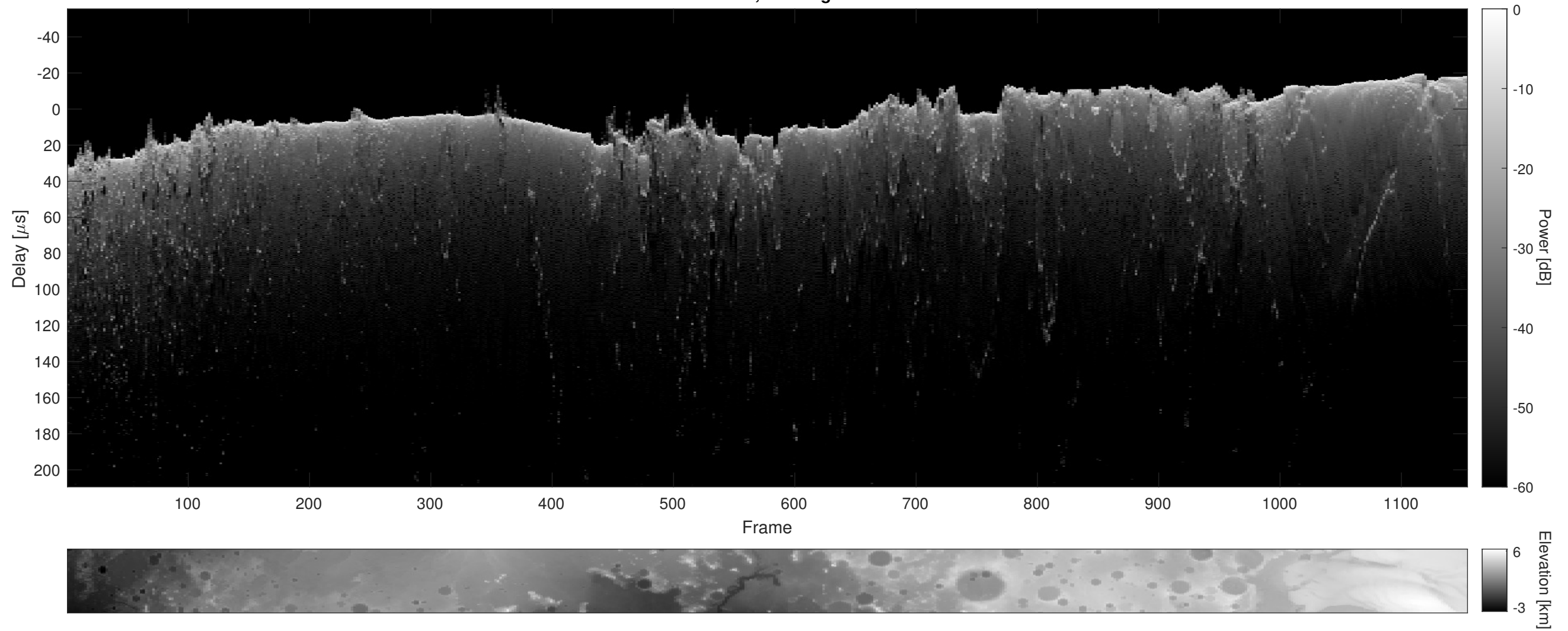
Orbit 4882, Cluttergram
