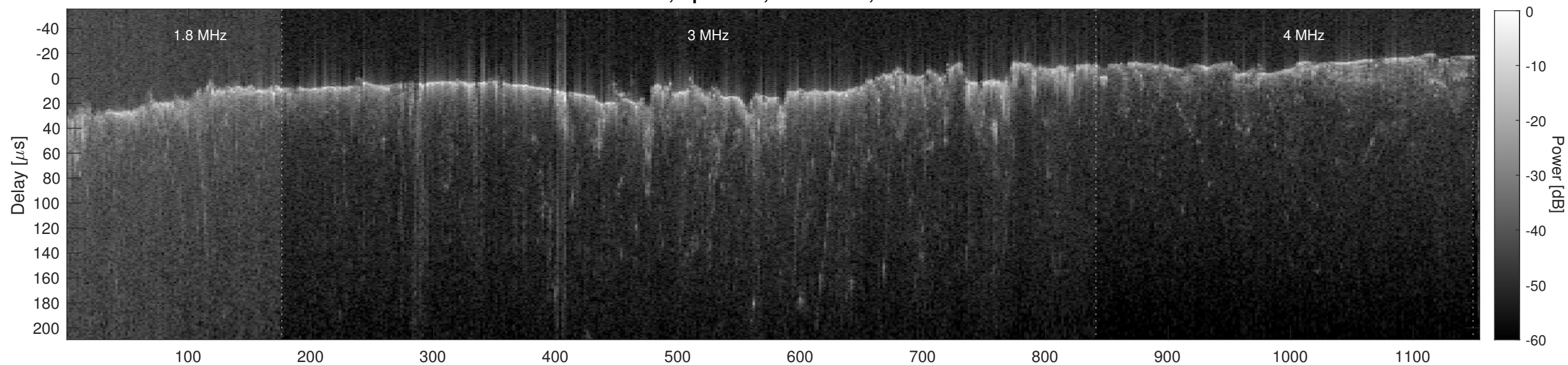
Orbit 4882, Cluttergram
