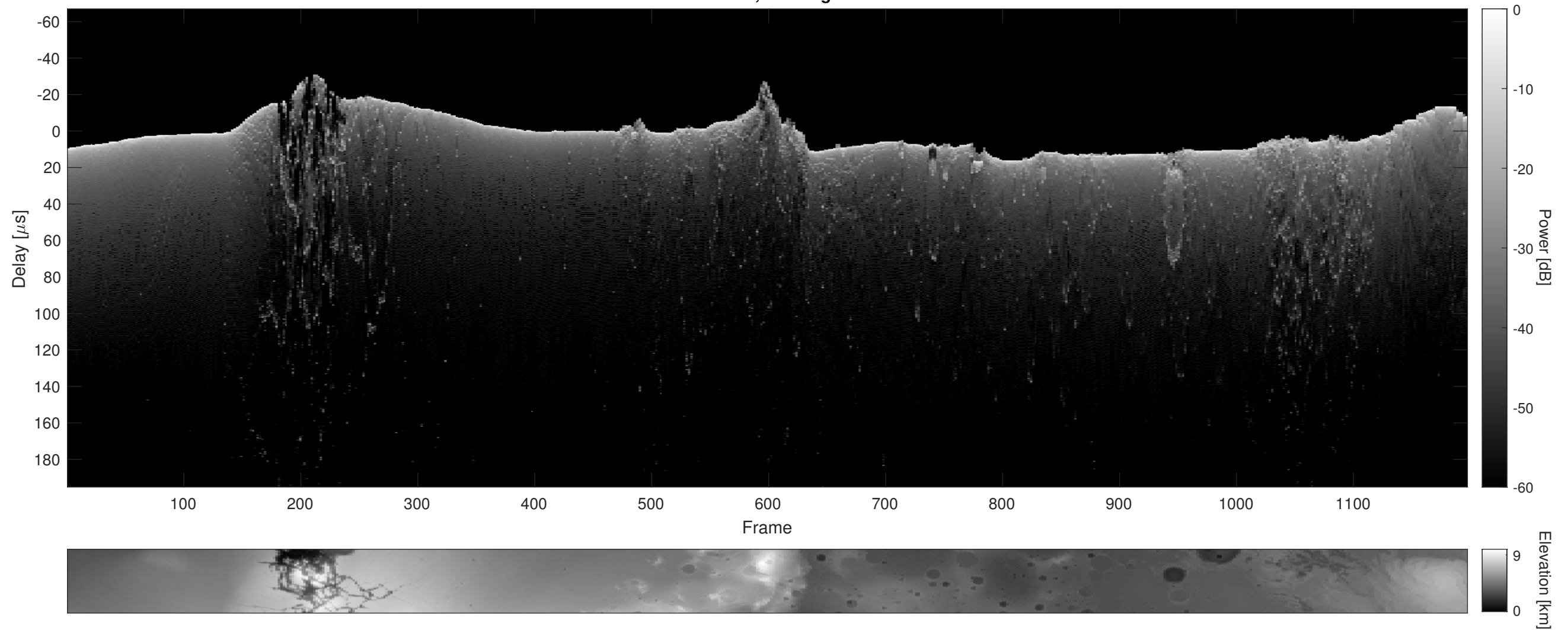
Orbit 4884, Cluttergram
