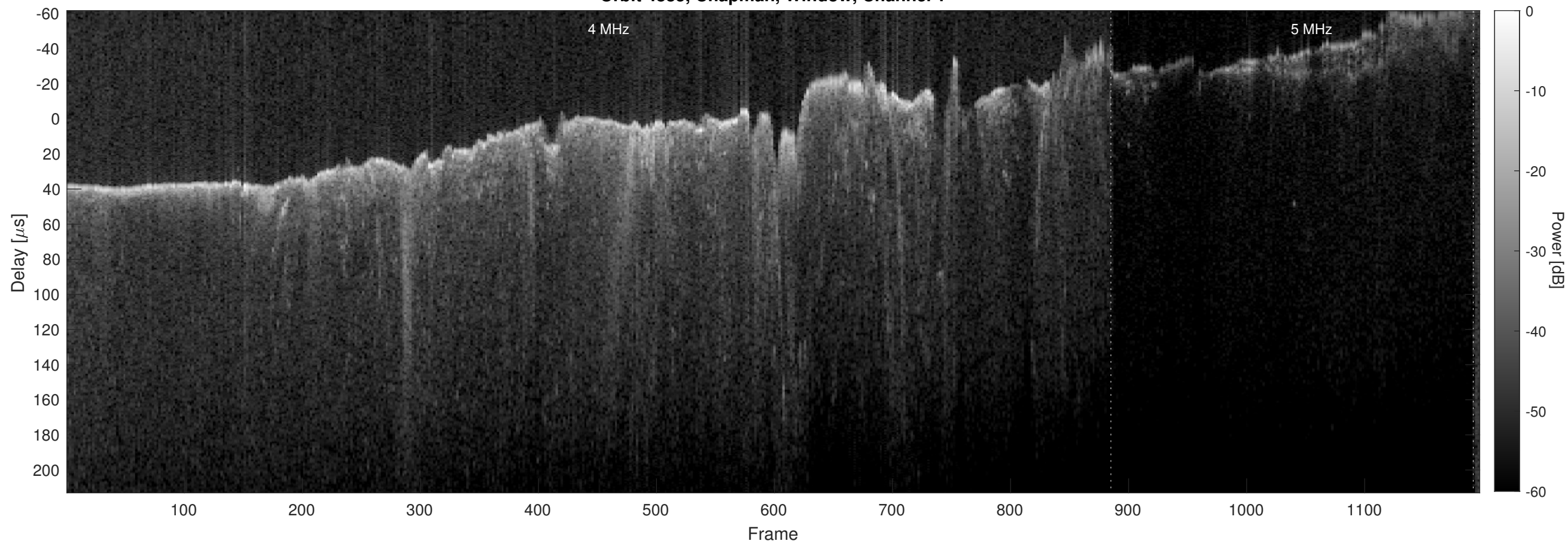
Orbit 4885, Chapman, Window, Channel 2
