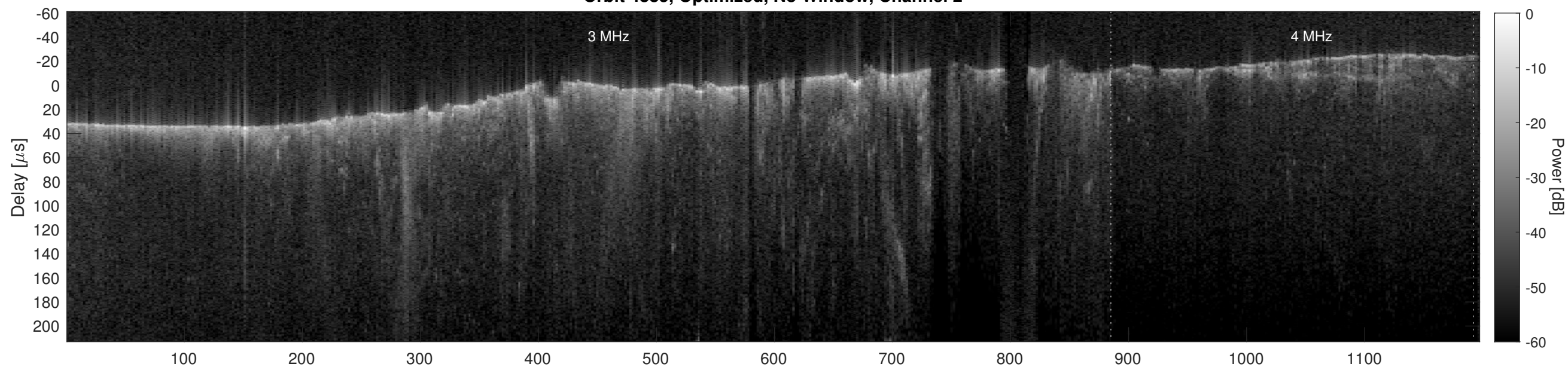
Orbit 4885, Cluttergram
