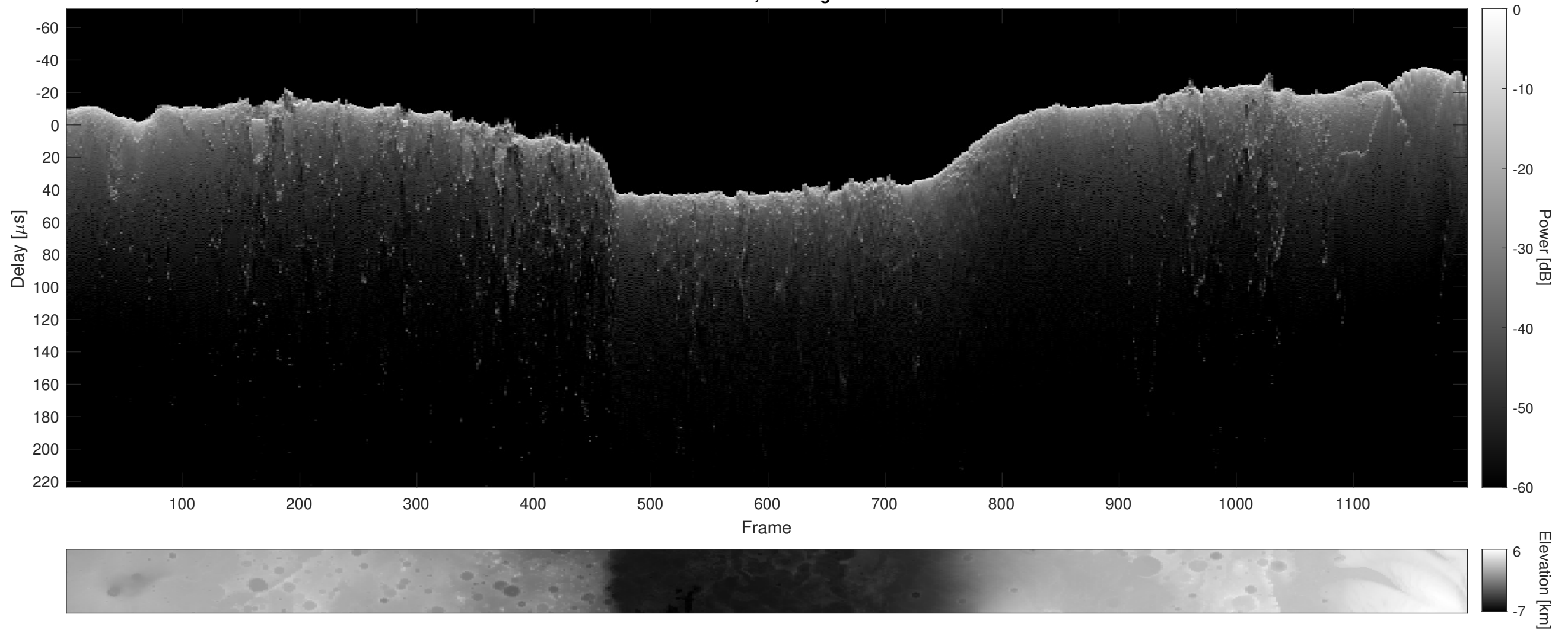
Orbit 4886, Cluttergram
