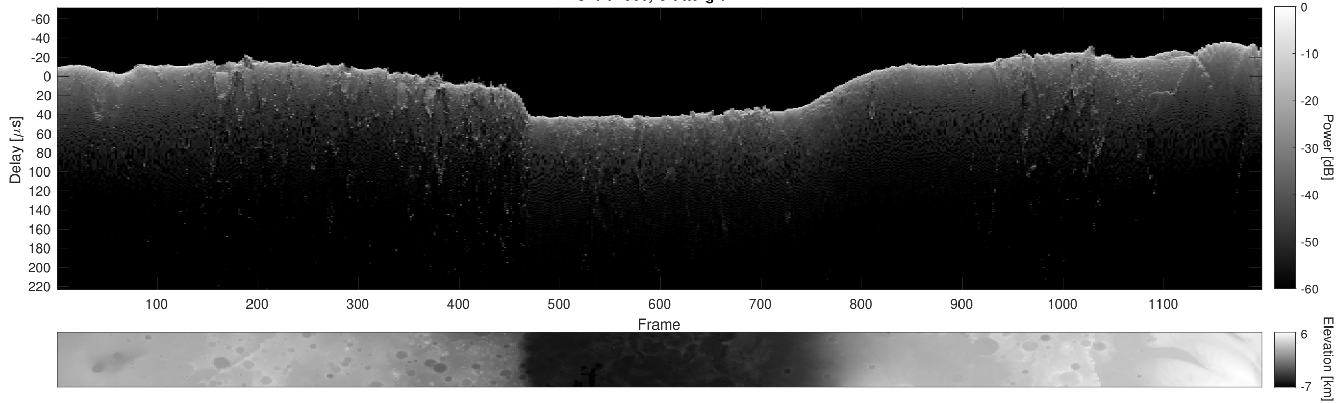
Orbit 4886, Cluttergram
