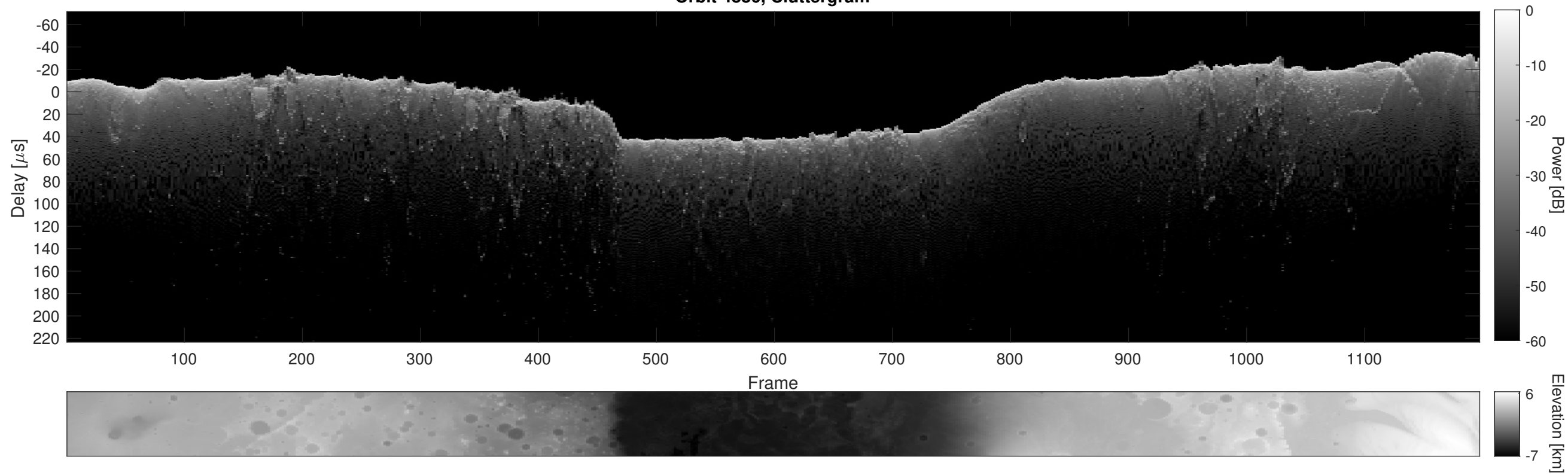
Orbit 4886, Cluttergram
