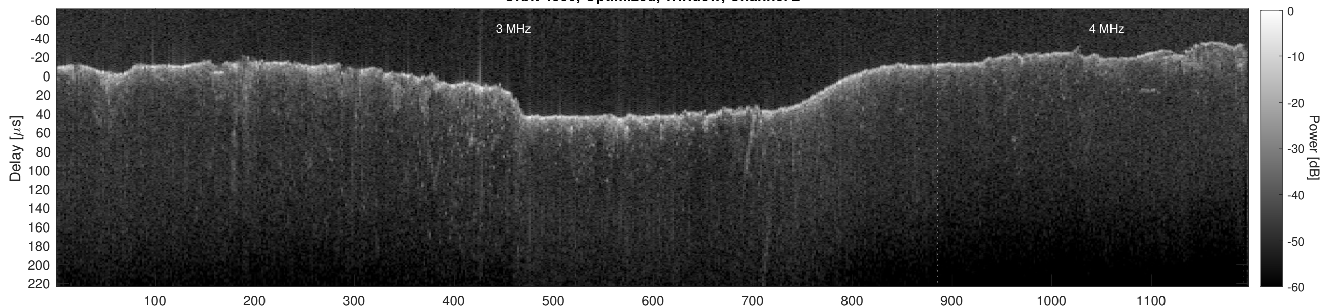
Orbit 4886, Cluttergram
