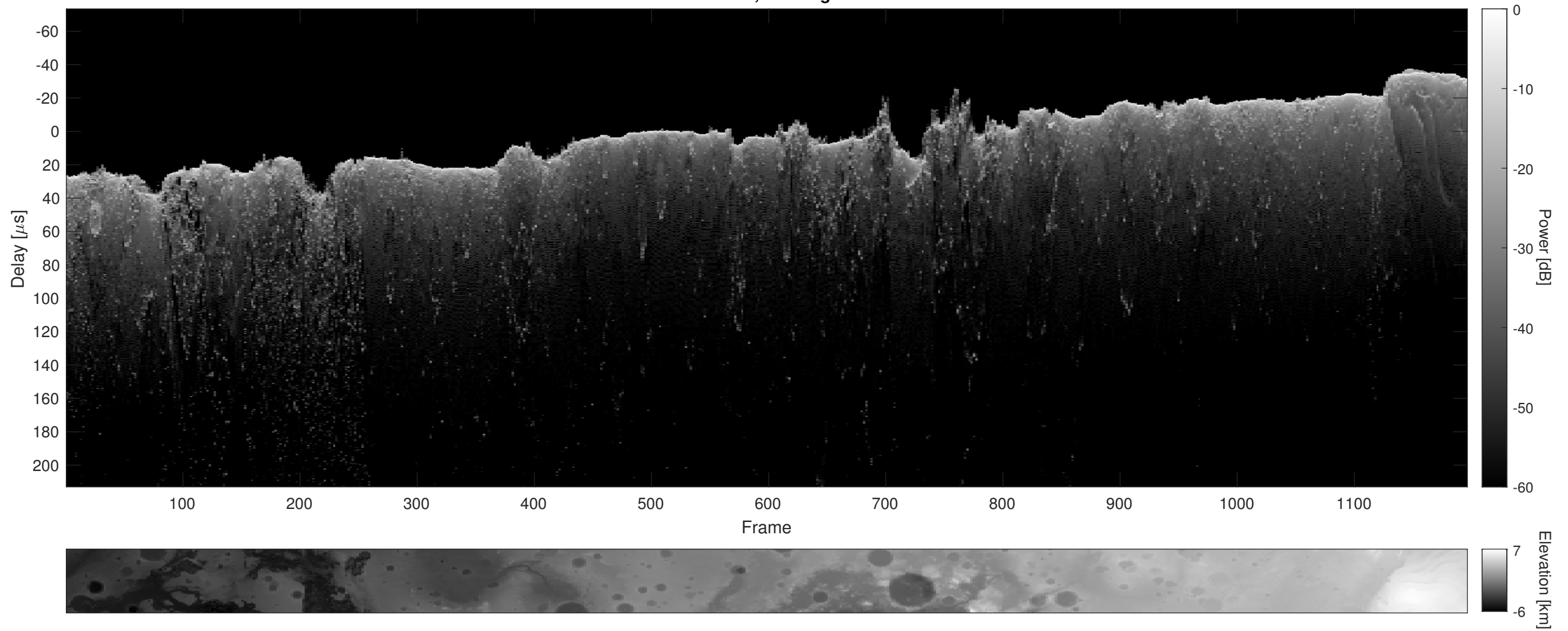
Orbit 4887, Cluttergram
