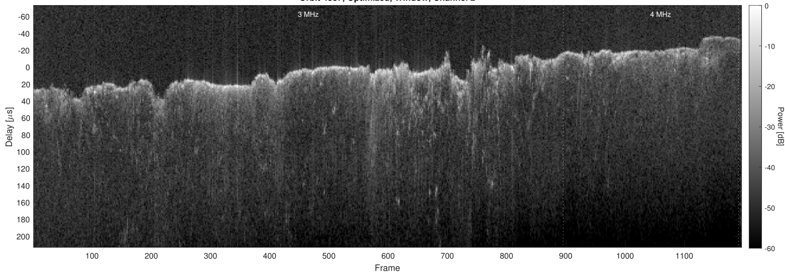
Orbit 4887, Optimized, Window, Channel 2
