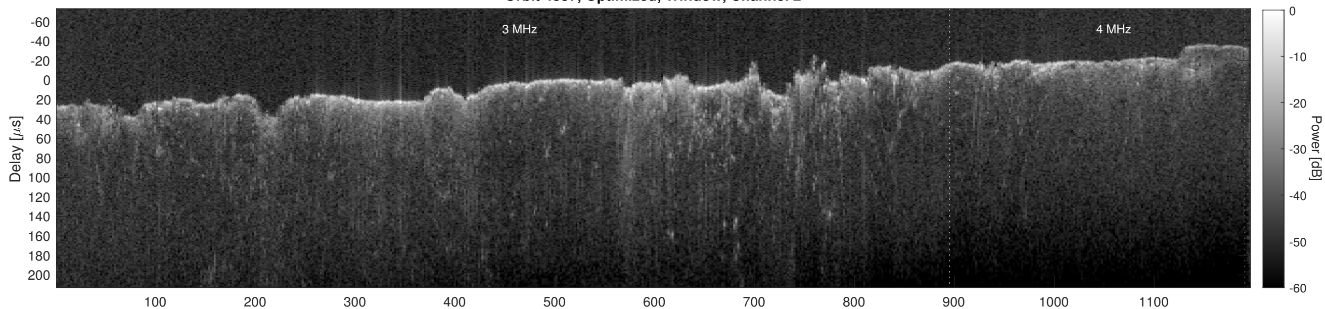
Orbit 4887, Cluttergram
