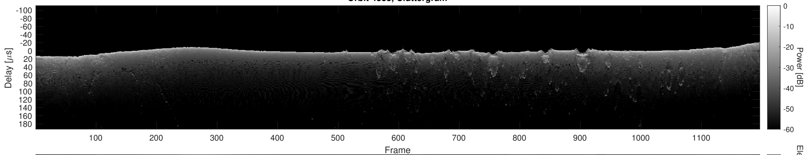
Orbit 4888, Cluttergram
