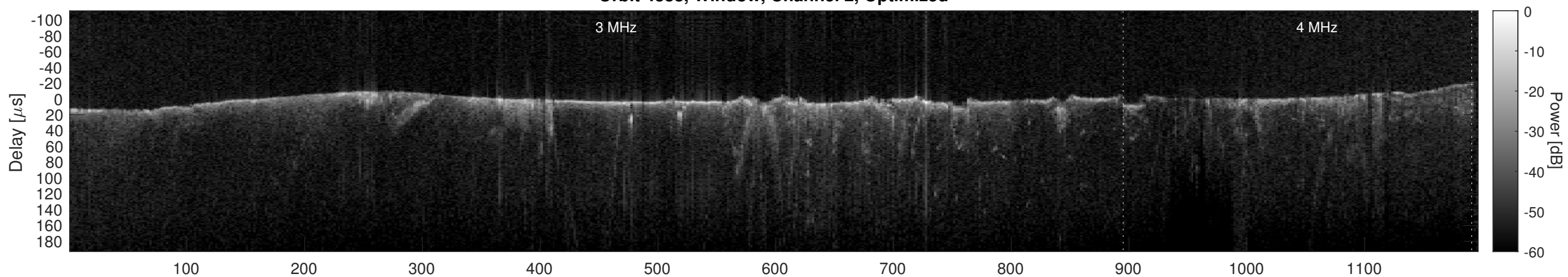
Orbit 4888, Cluttergram
