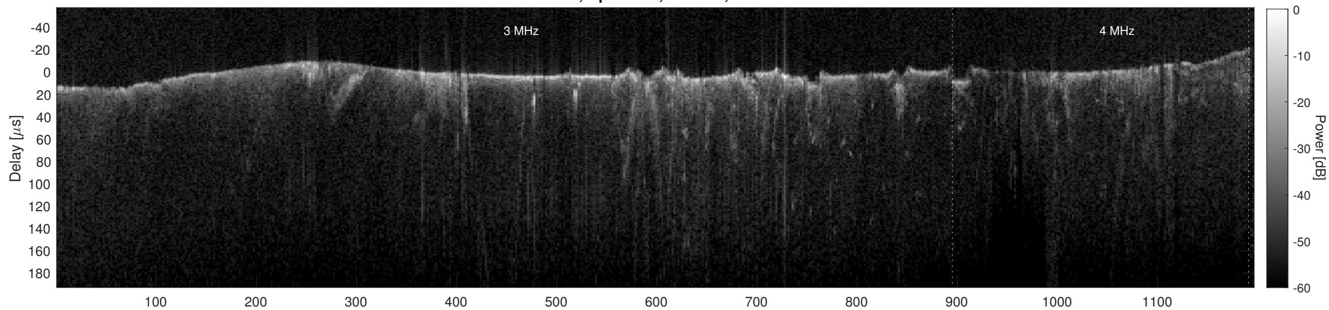
Orbit 4888, Cluttergram
