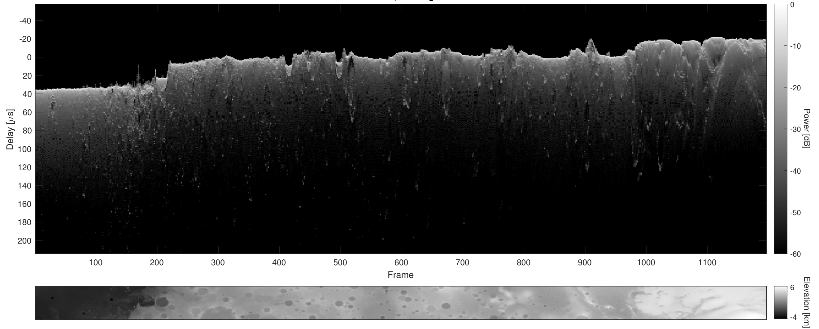
Orbit 4889, Cluttergram
