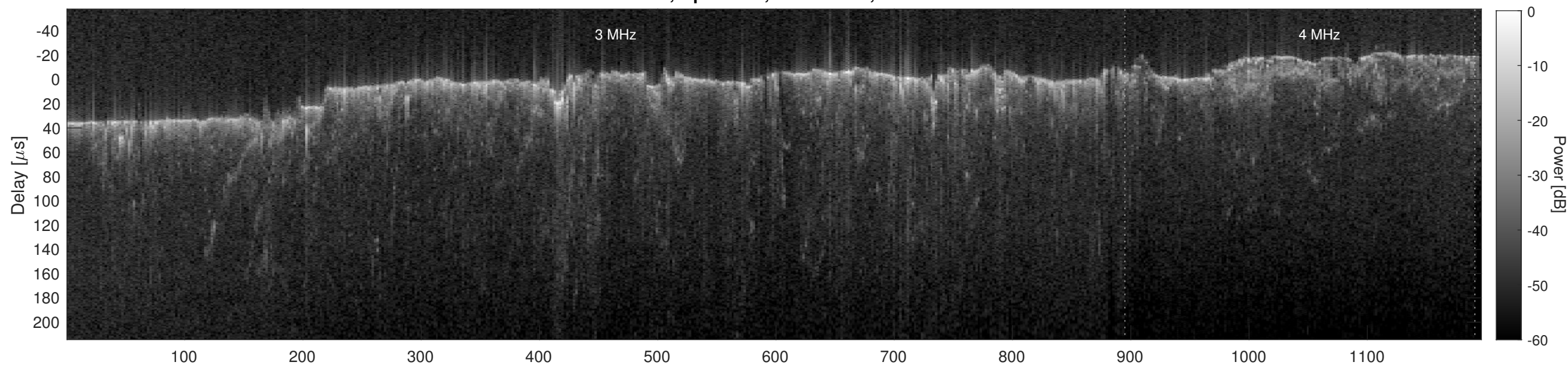
Orbit 4889, Cluttergram
