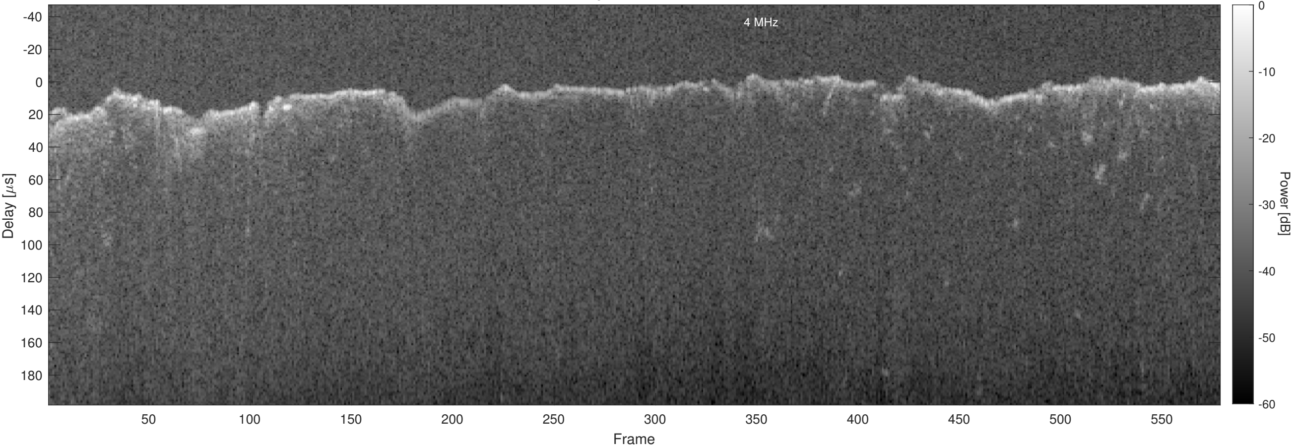
Orbit 4890, Chapman, Window, Channel 2
