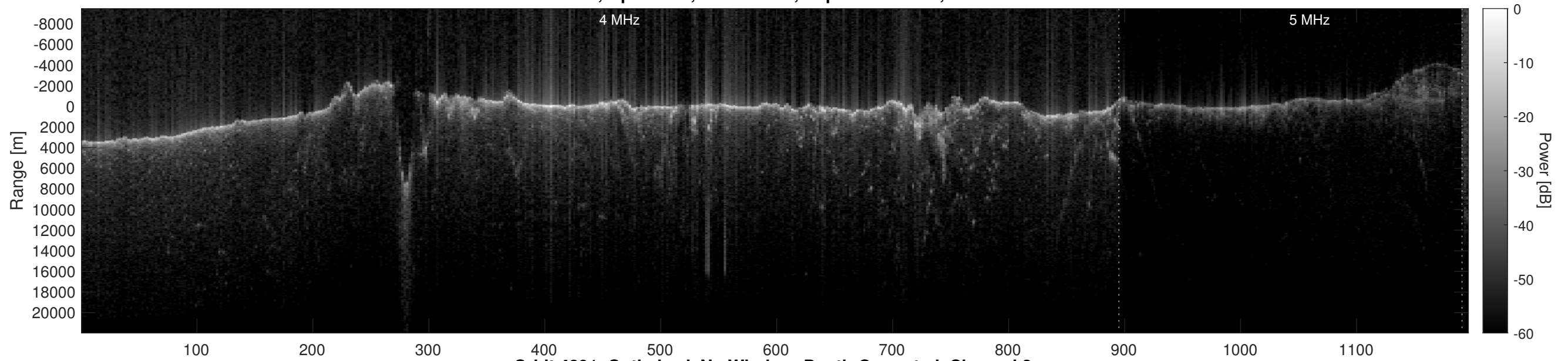
Orbit 4891, Optimized, No Window, Depth-Corrected, Channel 2
