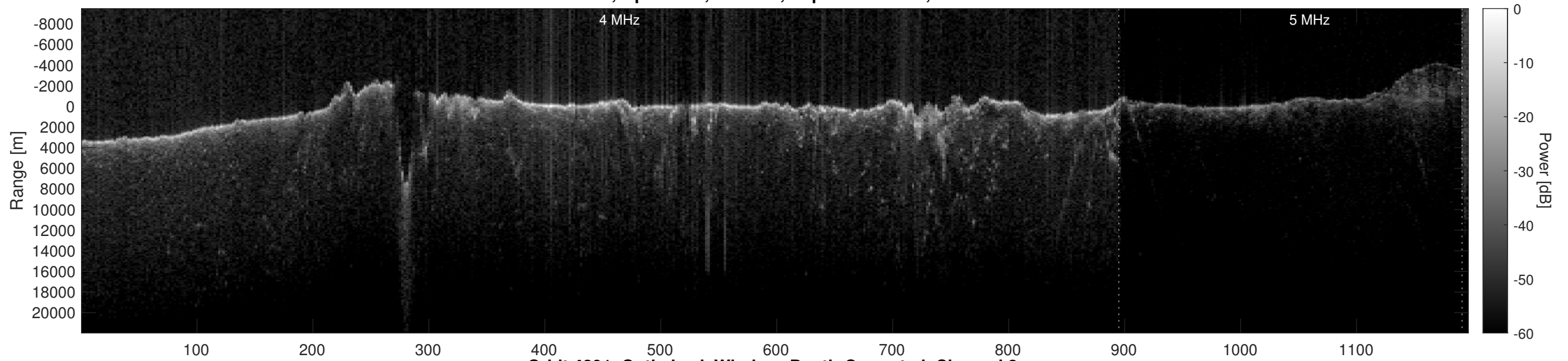
Orbit 4891, Optimized, Window, Depth-Corrected, Channel 2
