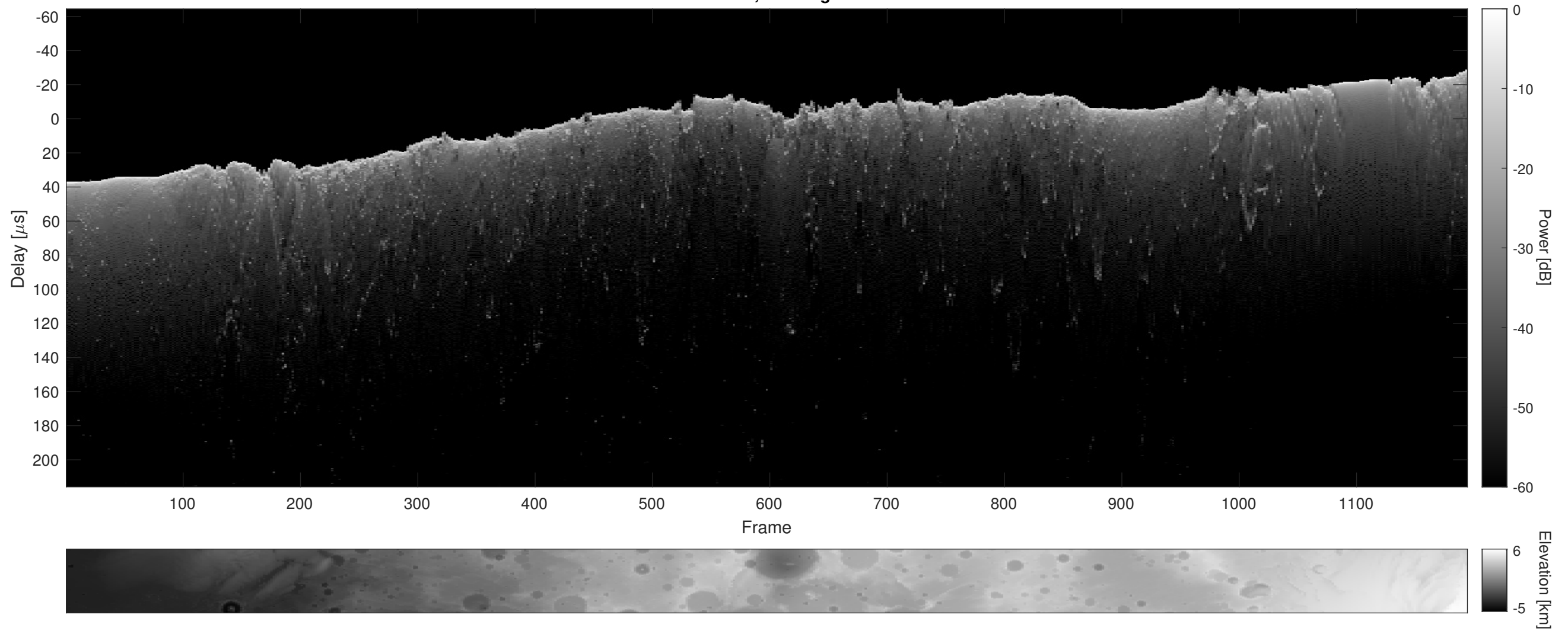
Orbit 4892, Cluttergram
