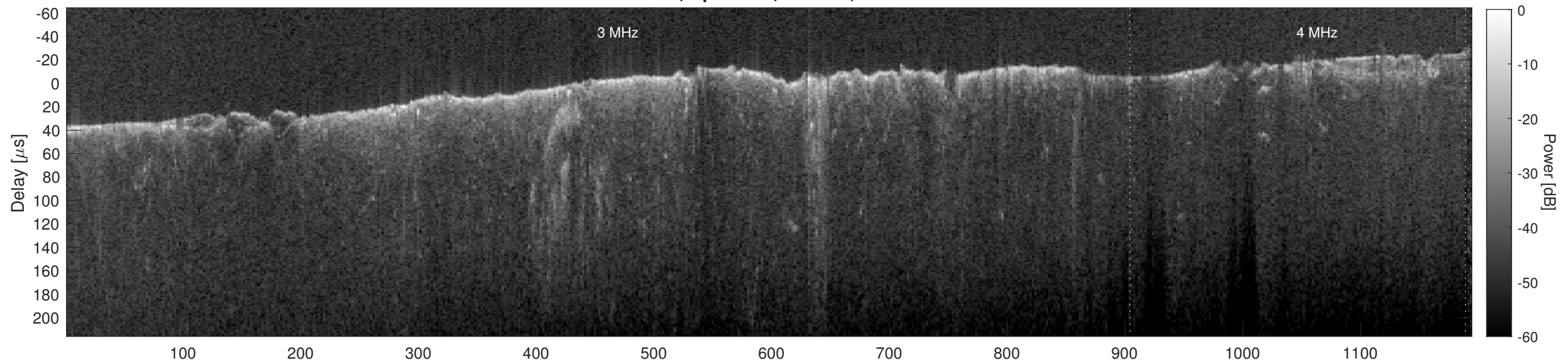
Orbit 4892, Cluttergram
