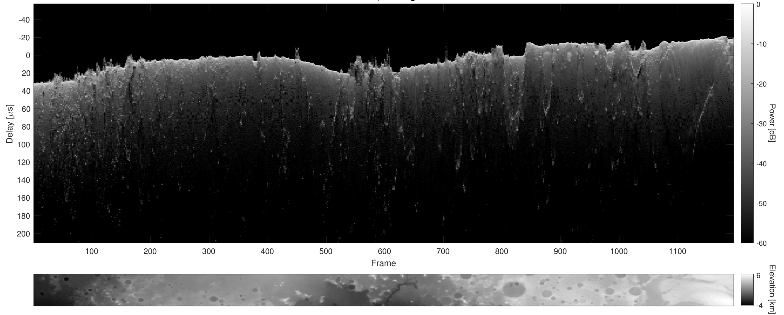
Orbit 4893, Cluttergram
