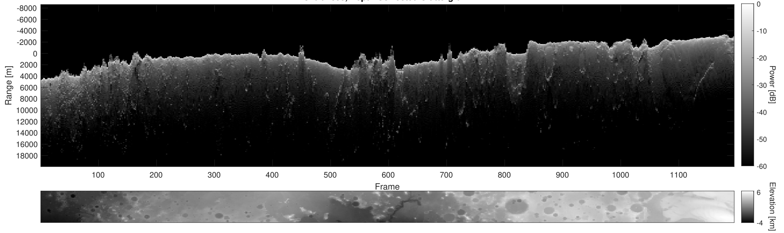
Orbit 4893, Depth-Corrected Cluttergram
