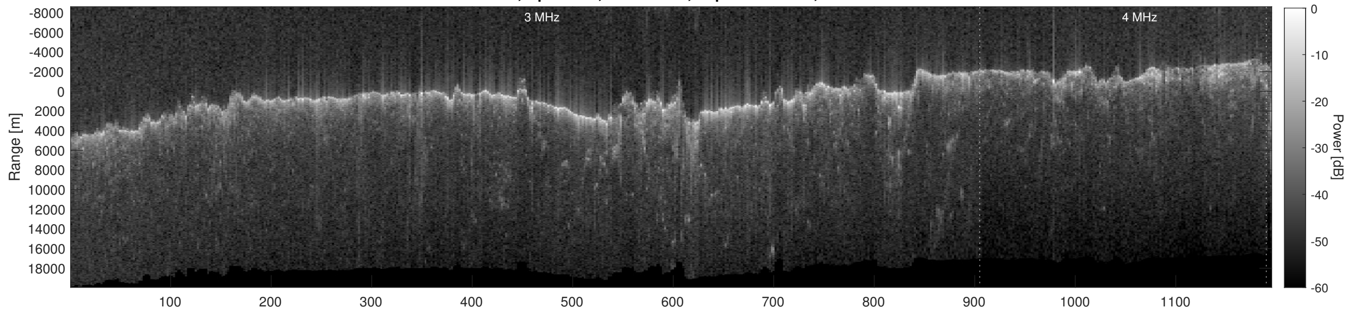
Orbit 4893, Depth-Corrected Cluttergram
