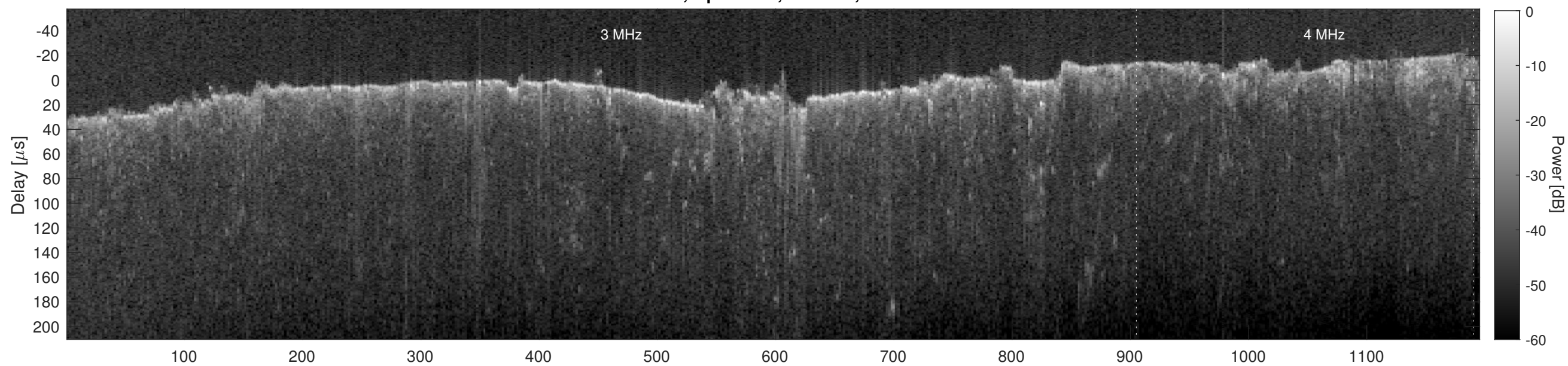
Orbit 4893, Cluttergram
