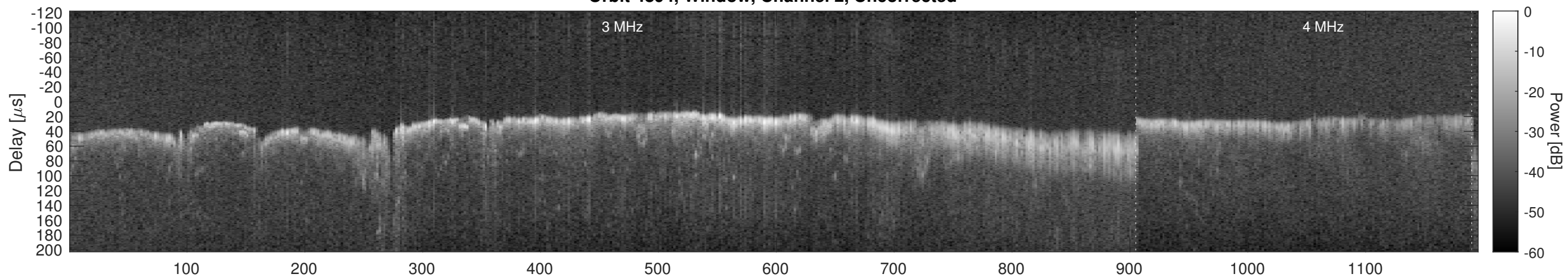
Orbit 4894, Window, Channel 2, Chapman
