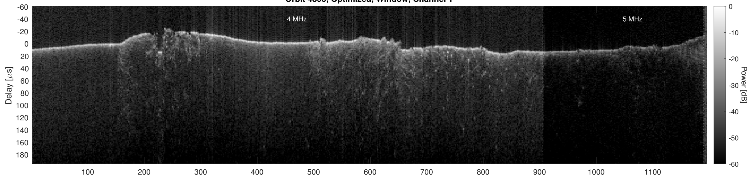
Orbit 4895, Optimized, Window, Channel 2
