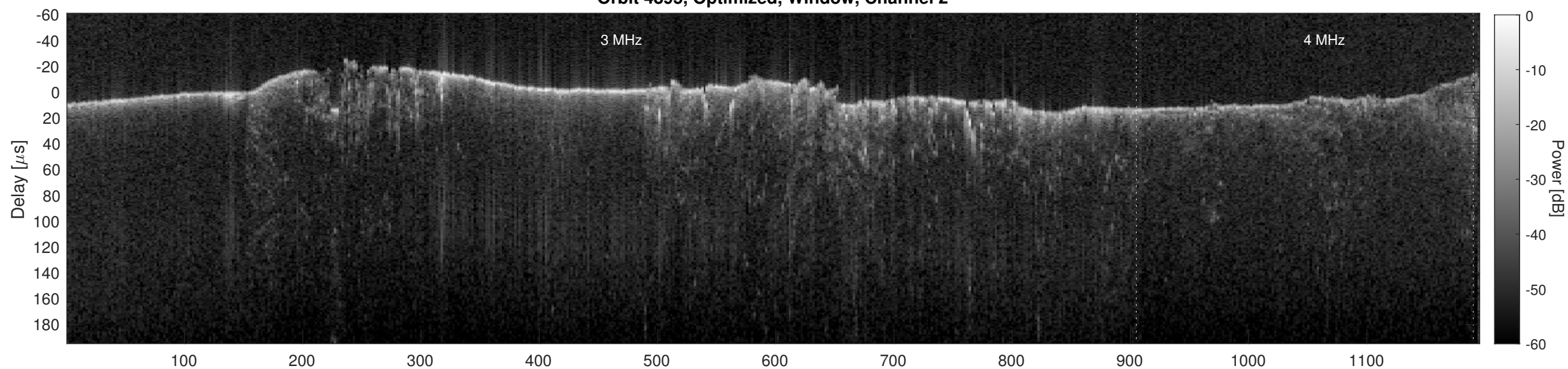
Orbit 4895, Cluttergram
