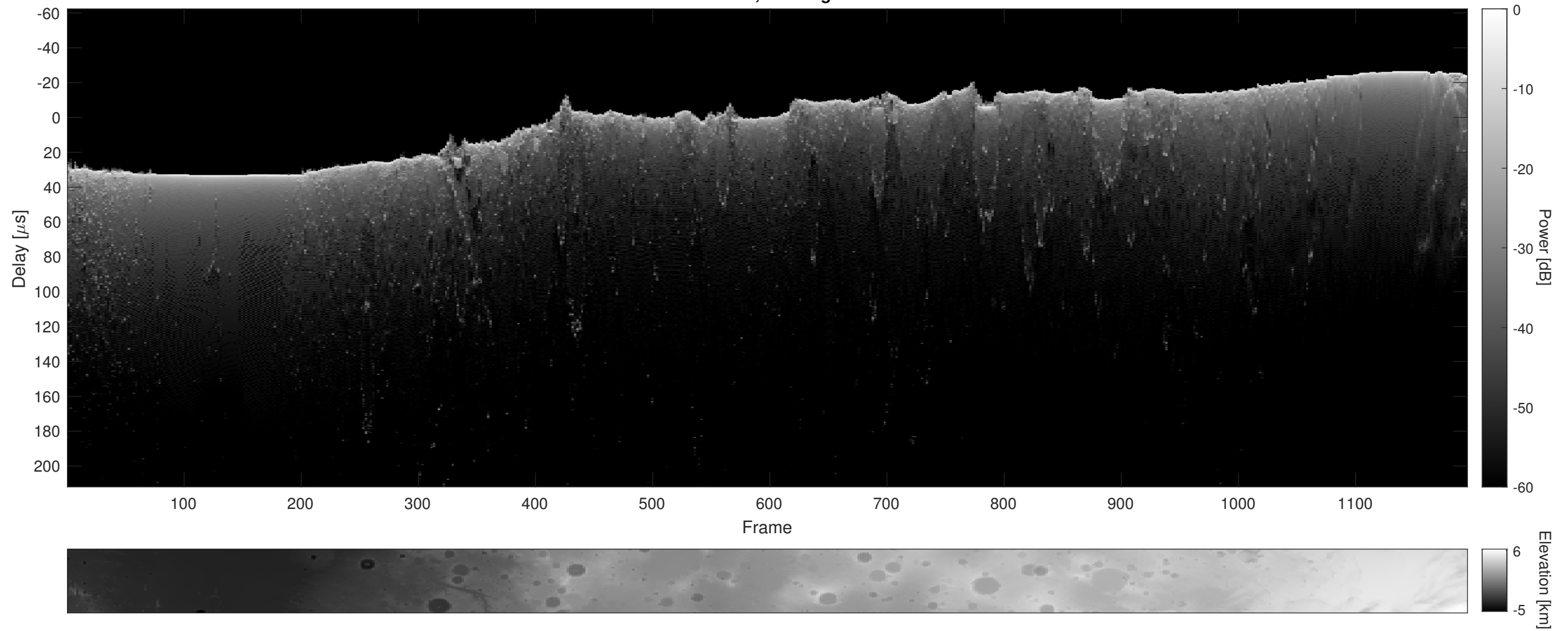
Orbit 4896, Cluttergram
