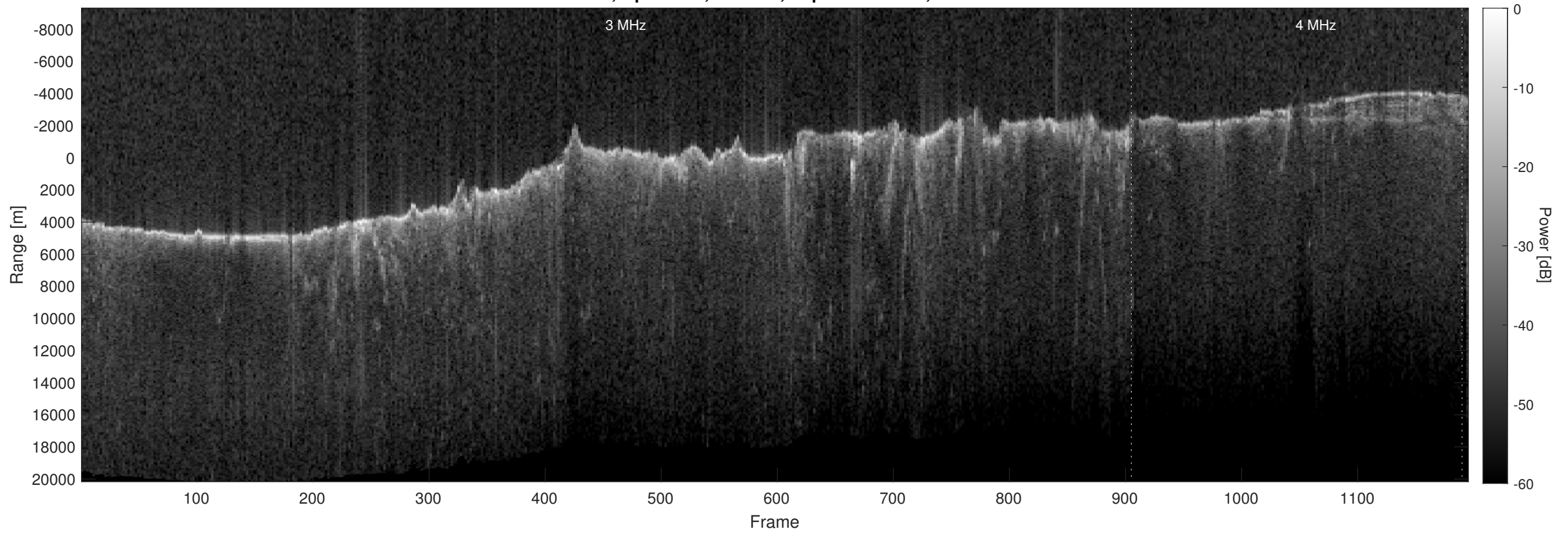
Orbit 4896, Optimized, Window, Depth-Corrected, Channel 2
