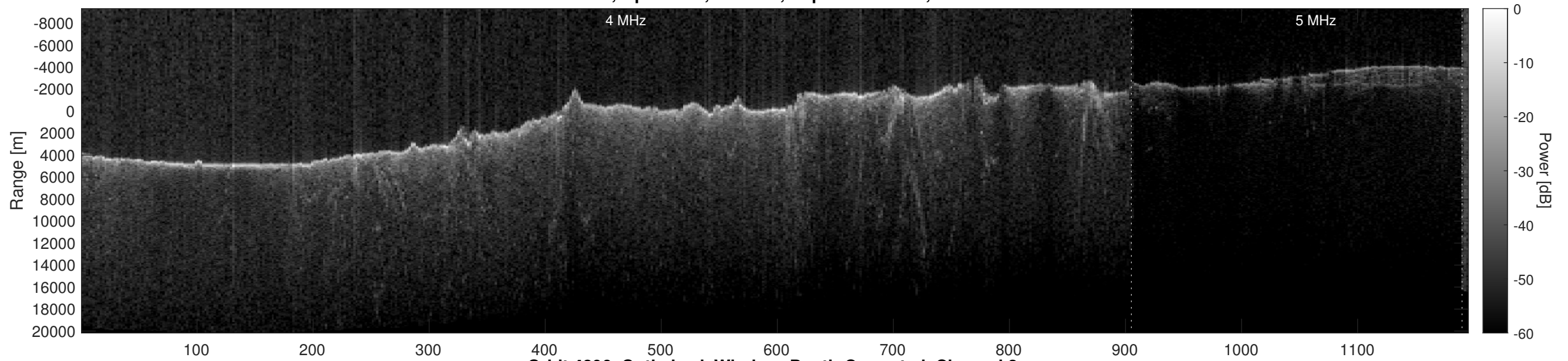
Orbit 4896, Optimized, Window, Depth-Corrected, Channel 2
