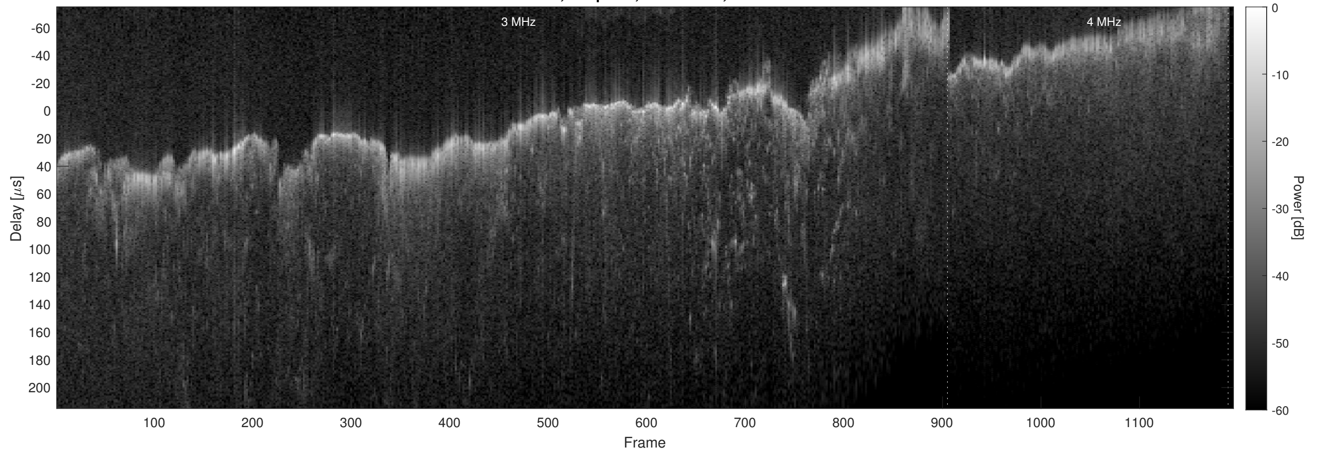
Orbit 4898, Chapman, No Window, Channel 2
