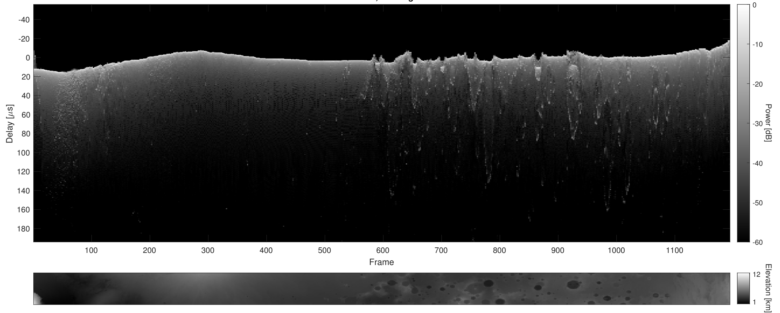
Orbit 4899, Cluttergram
