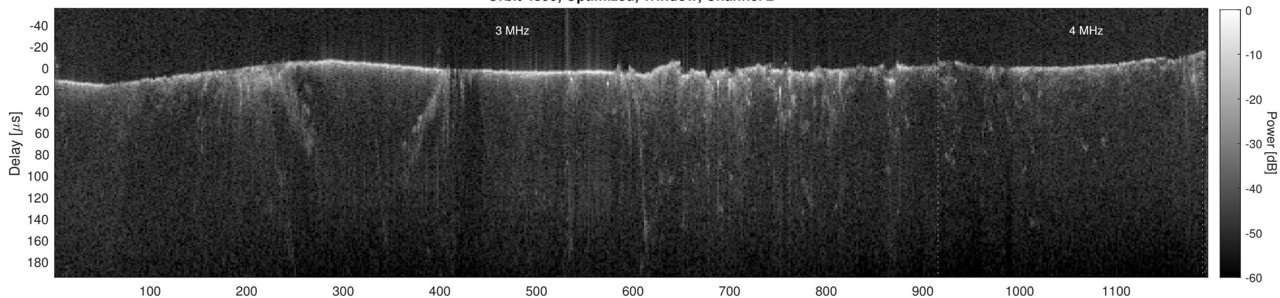
Orbit 4899, Cluttergram
