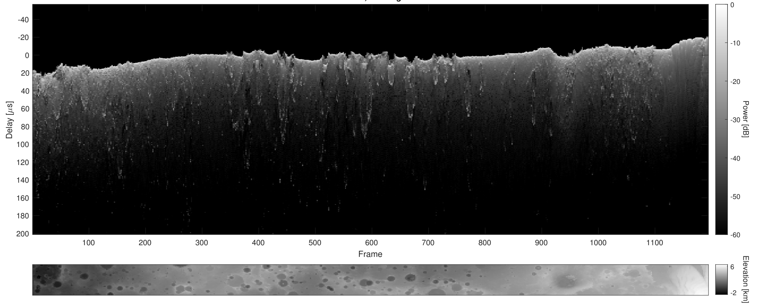
Orbit 4901, Cluttergram
